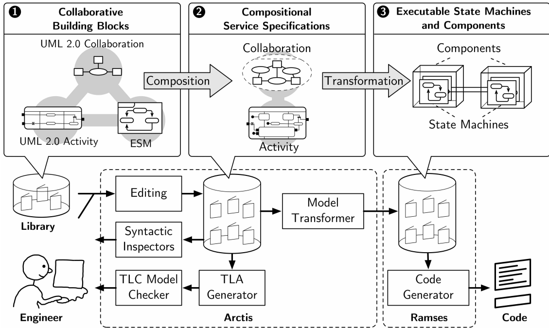
Fig. 1. A coarse sketch of the SPACE engineering approach and its tool support
